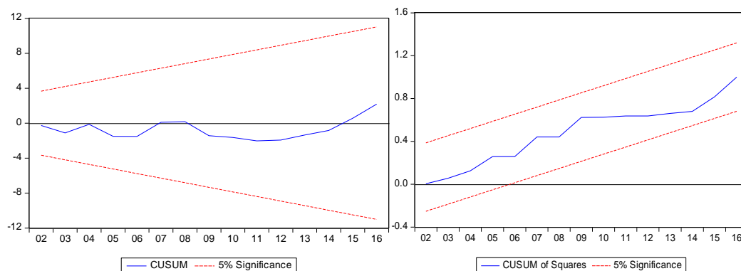
Figure 1: CUSUM and CUSUM Square Parameter Stability Tests
